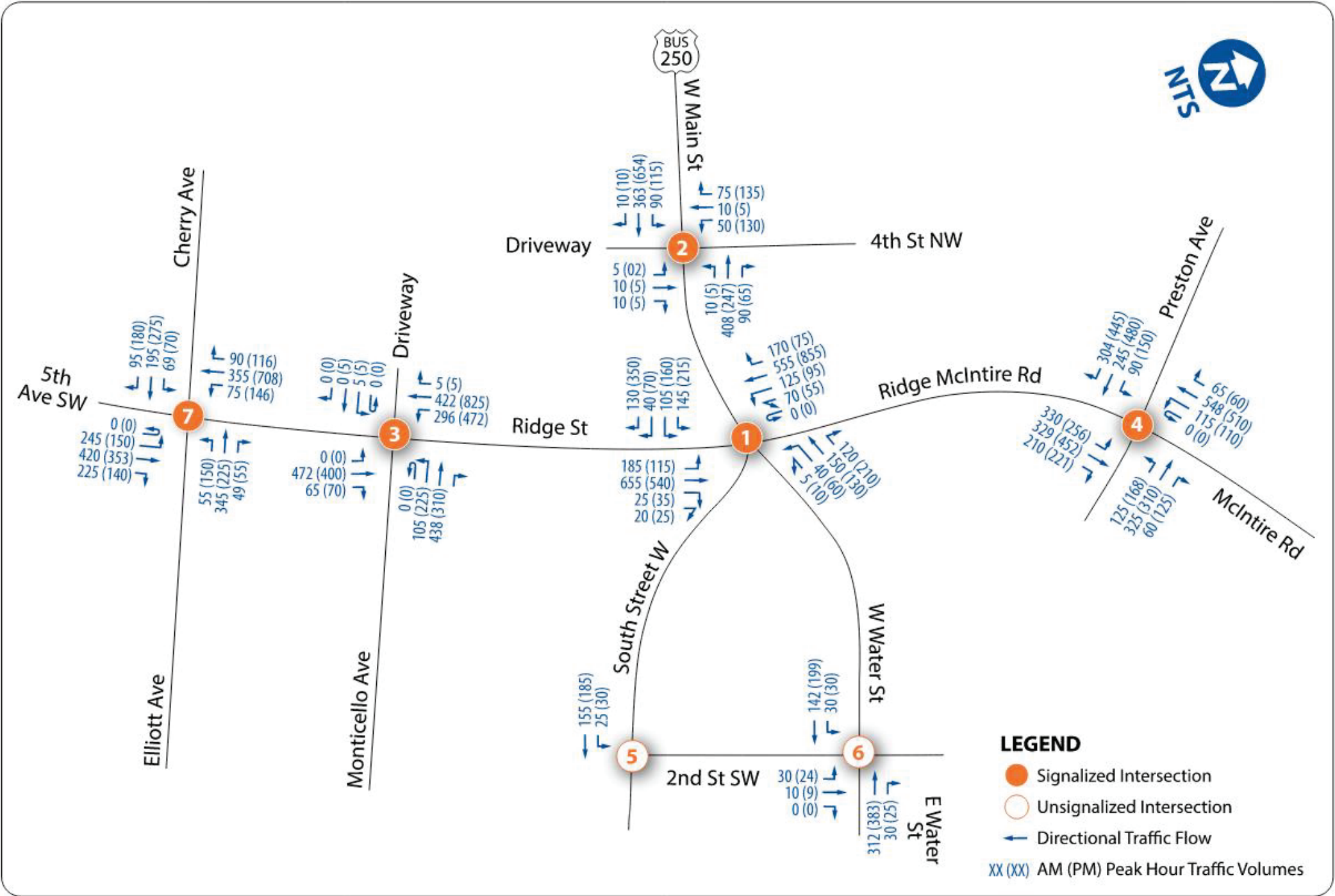
Figure 19: Future Interim (2045) Balanced Peak Hour Traffic Volumes
