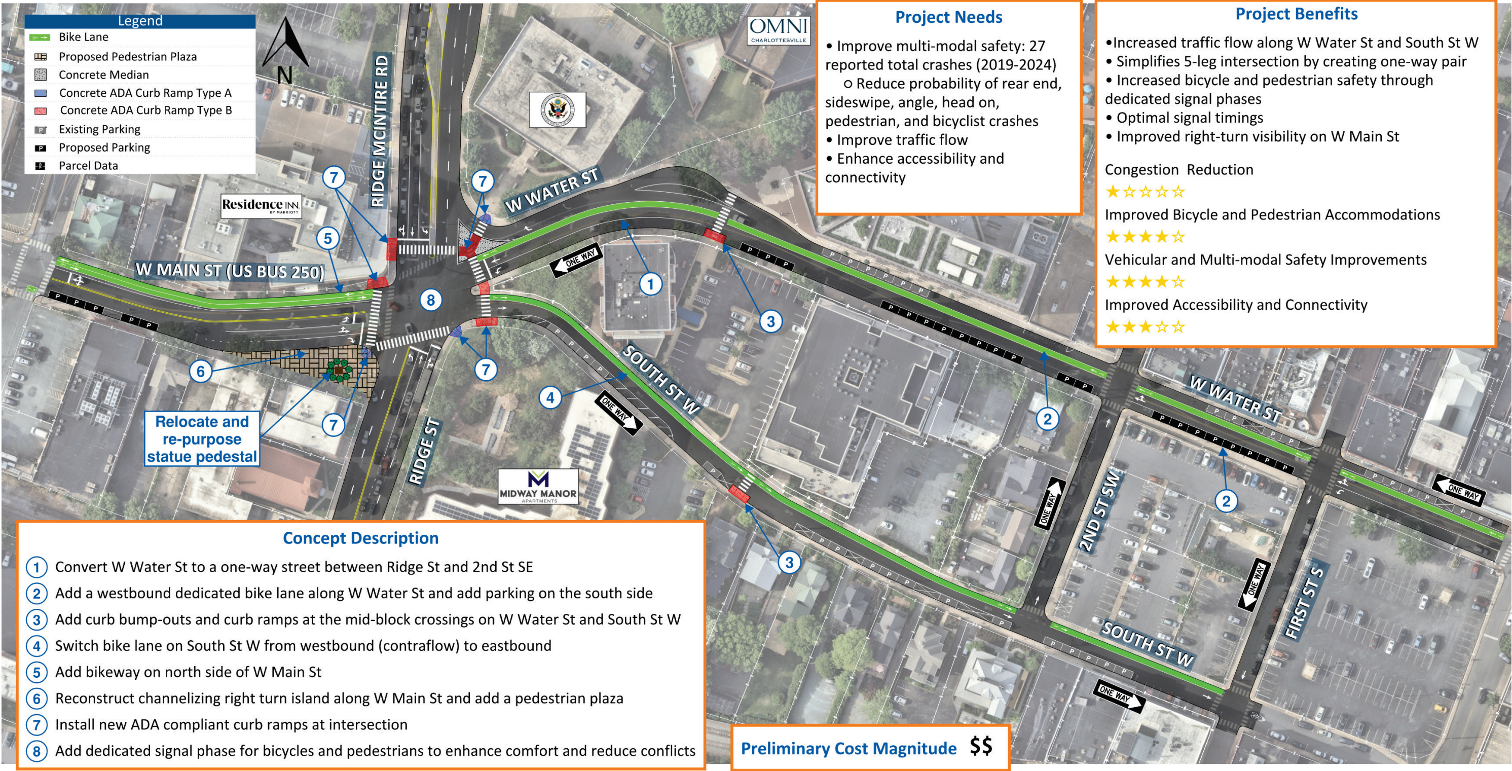
Figure 30: Preliminary Alternative 2 - One-way Pair for Water St and South St with Bikeway
