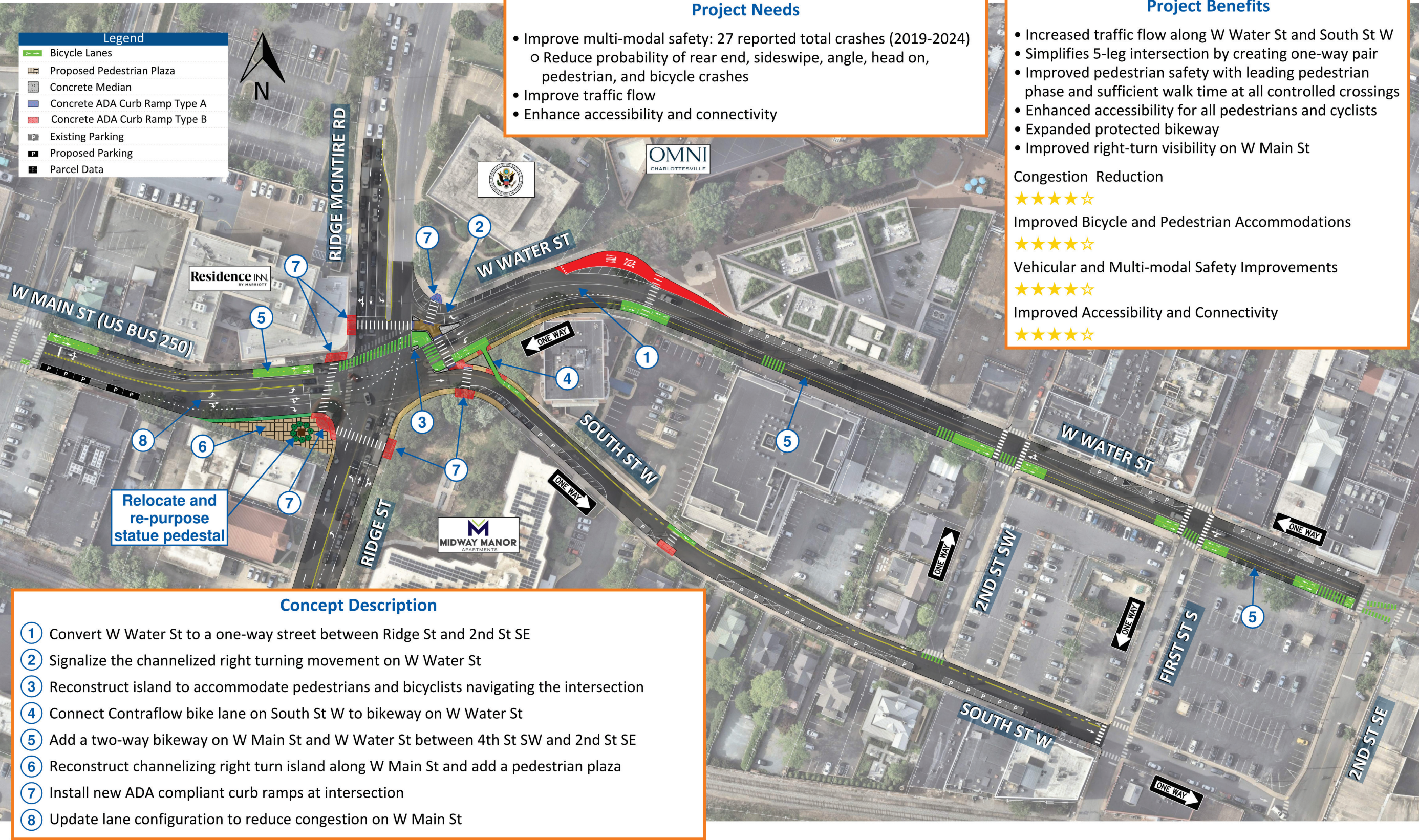
Figure 32: Preferred Alternative - One-way Pair for Water St and South St with Bikeway
