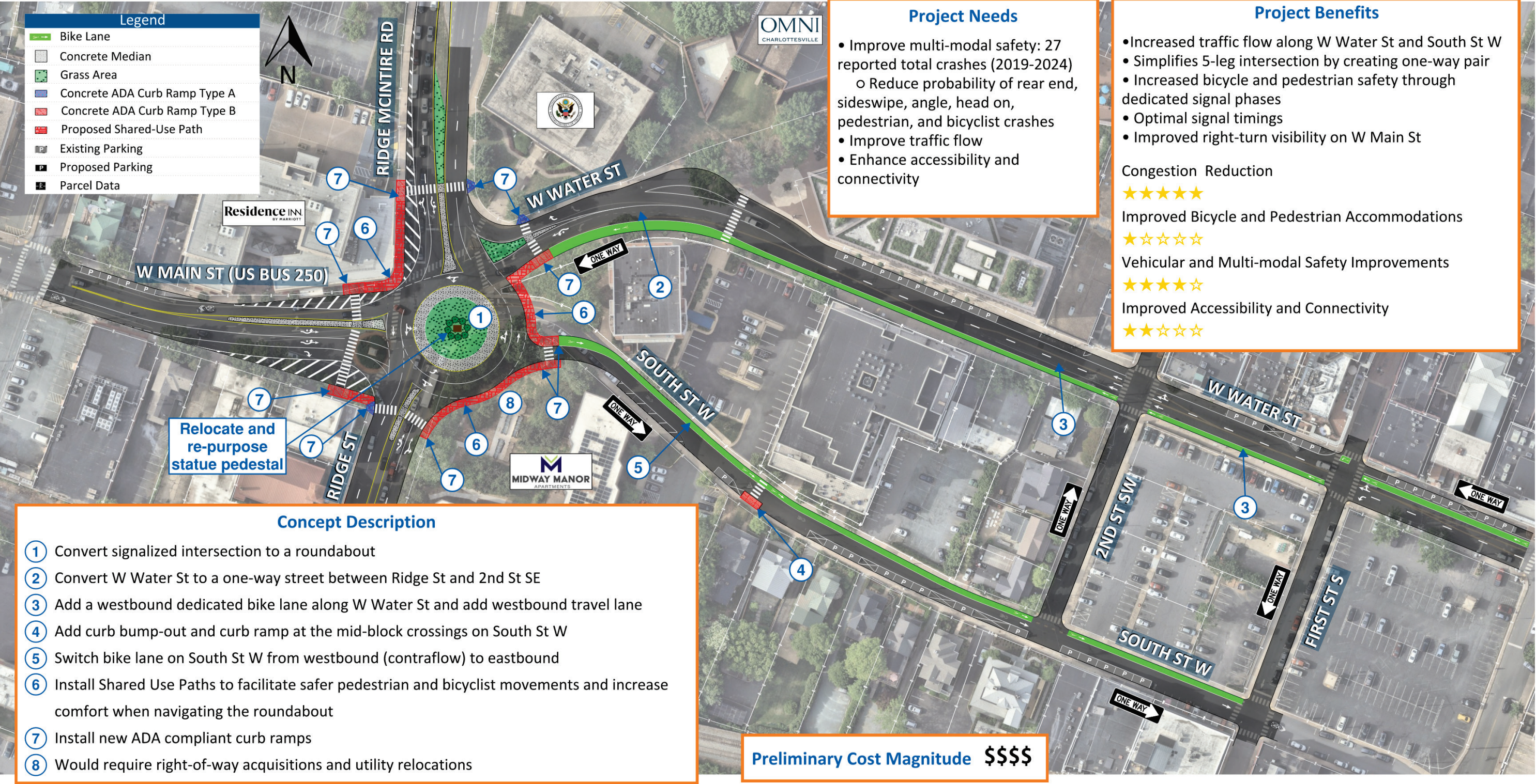
Figure 31: Preliminary Alternative 3 - Roundabout with One-way Pair for Water St and South St
